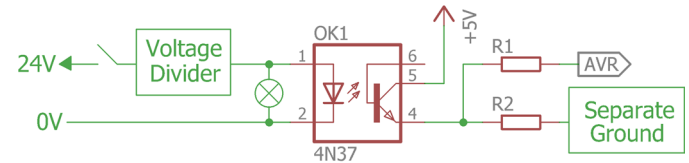
Fig. 2. Circuit diagram of PLC module input for the second prototype.
