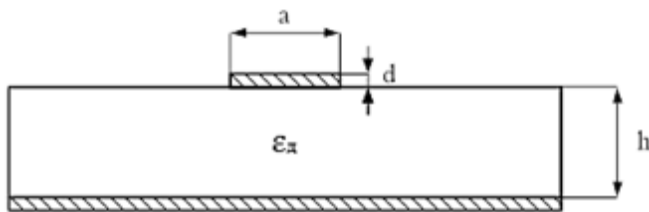
Fig. 3. Cross section of band asymmetric waveguide
