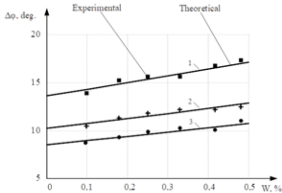
Fig. 7. Theoretical and experimental static characteristics of band-type asymmetric humidity sensor, for some values of informative waves' frequency: 1 –400 MHz; 2 – 300 MHz; 3 –250 MHz
