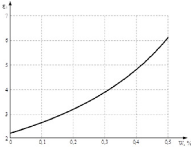
Fig. 2. Theoretical dependence between integral dielectric permittivity and sample's moisture content
